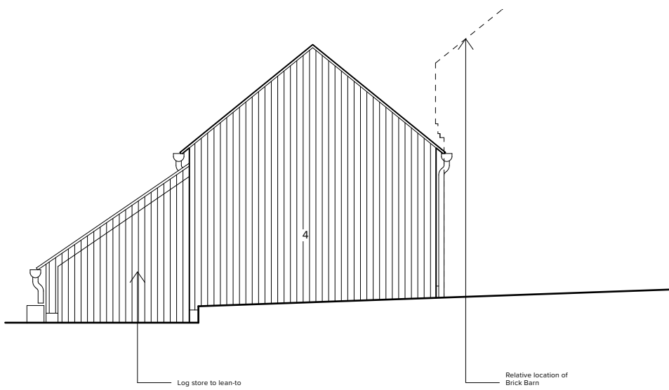
North Elevation
