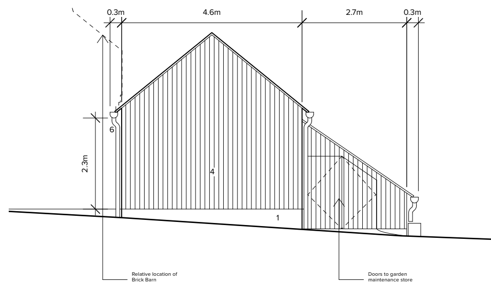
South Elevation
